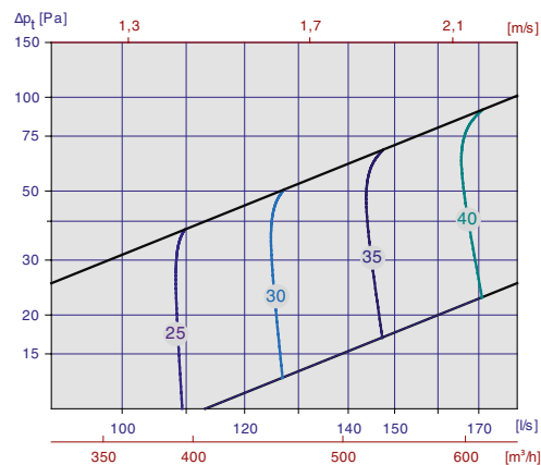
Diagram 15, Tilluft Orion-LØV m/Luna 315-315
