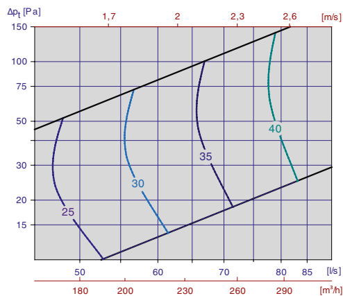
Diagram 9, Tilluft Orion-LØV m/Luna 200-200
