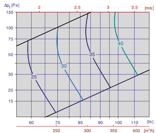
Diagram 10, Tilluft Orion-LØV m/Luna 200-250
