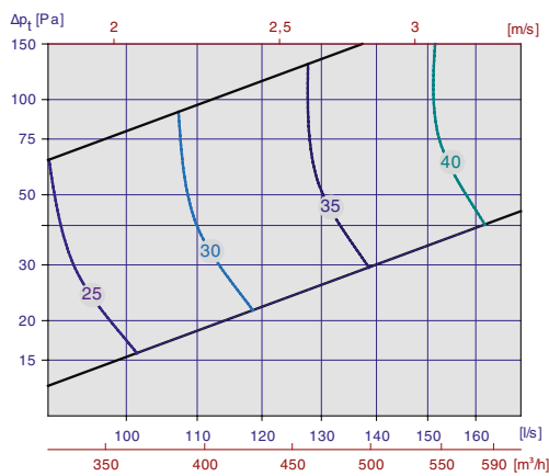
Diagram 13, Tilluft Orion-LØV m/Luna 250-315
