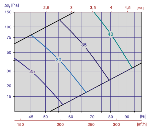
Diagram 8, Tilluft Orion-LØV m/Luna 160-250
