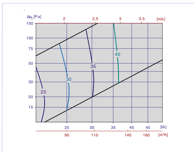
Diagram 3, Tilluft Orion-LØV m/Luna 125-125
