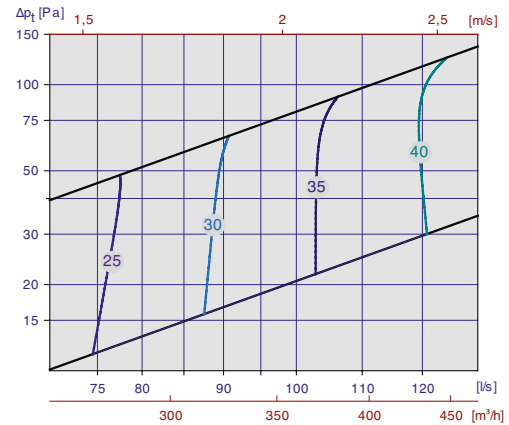
Diagram 12, Tilluft Orion-LØV m/Luna 250-250
