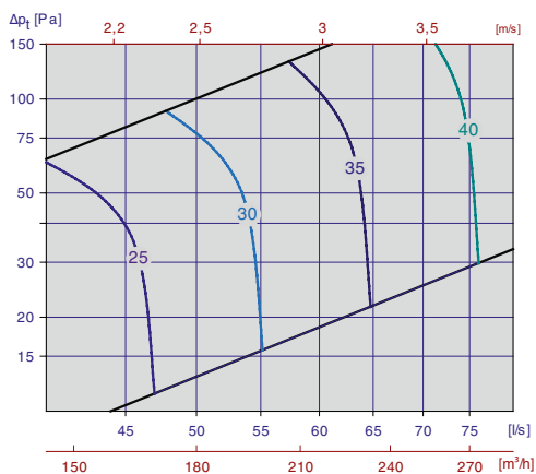
Diagram 7, Tilluft Orion-LØV m/Luna 160-200
