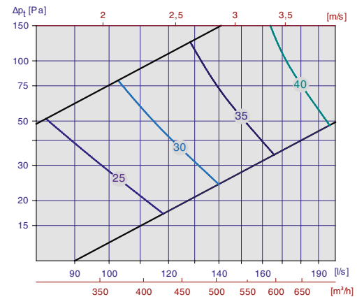
Diagram 14, Tilluft Orion-LØV m/Luna 250-400
