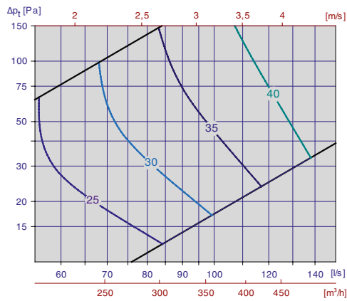
Diagram 11, Tilluft Orion-LØV m/Luna 200-315
