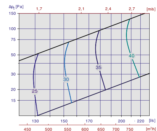
Diagram 16, Tilluft Orion-LØV m/Luna 315-400
