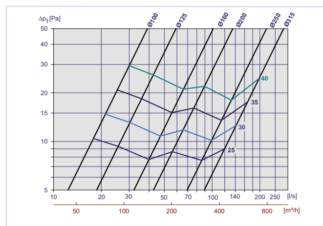
Diagram 17, Tilluft kapasitetsdiagram for LØV-R i 90° bend.
