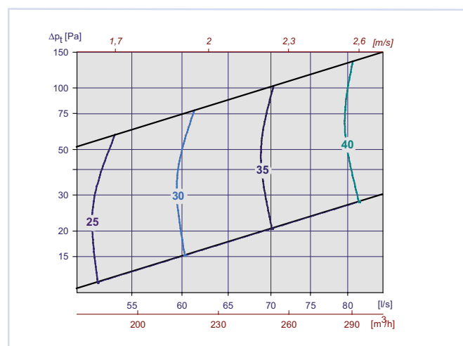
Diagram 10, Tilluft LØV-R m/Luna 200-200
